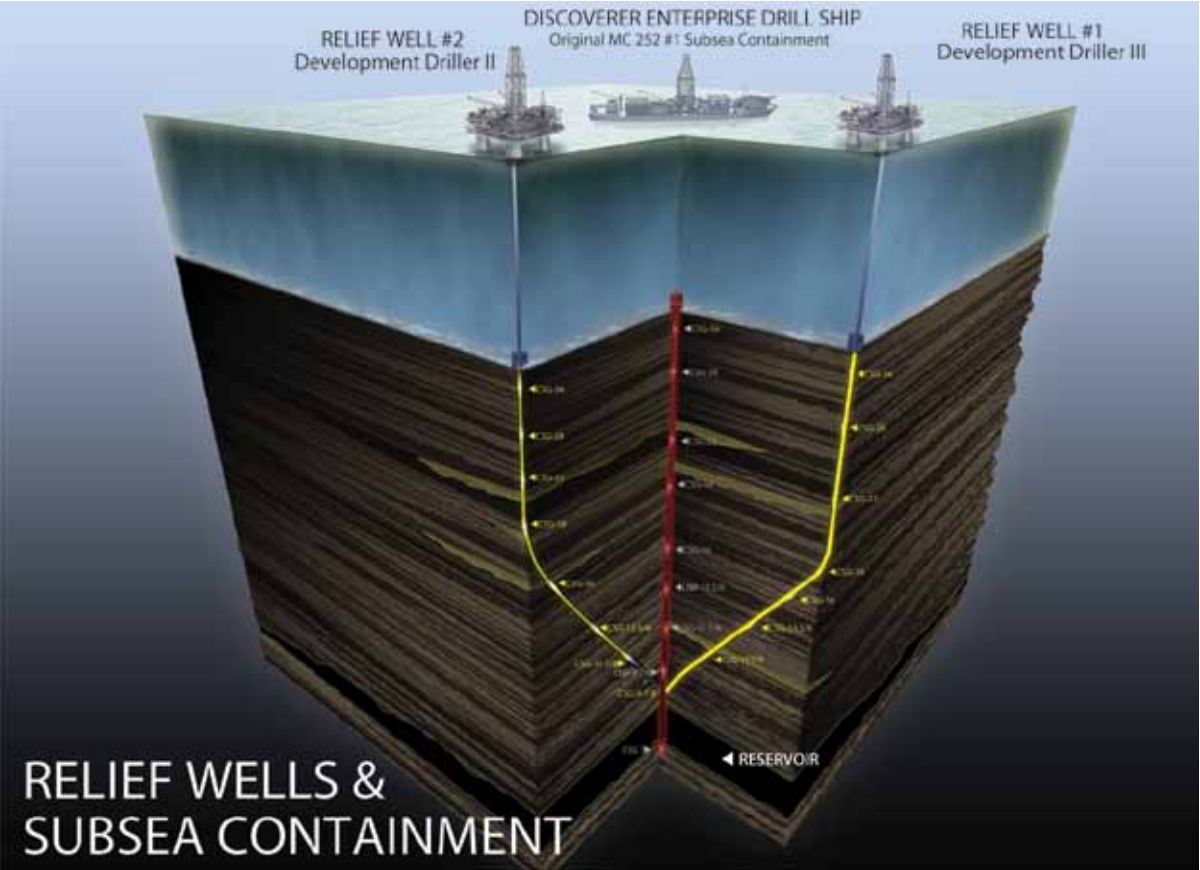
The drilling of two relief wells was part of the containment plan for ensuring final “kill” of the Deepwater Horizon well. A dedicated relief well operation was stood up and rapidly took innovative steps allowing the drilling of a relief well to within 30 to 50 feet of intercept in approximately 100 days.
