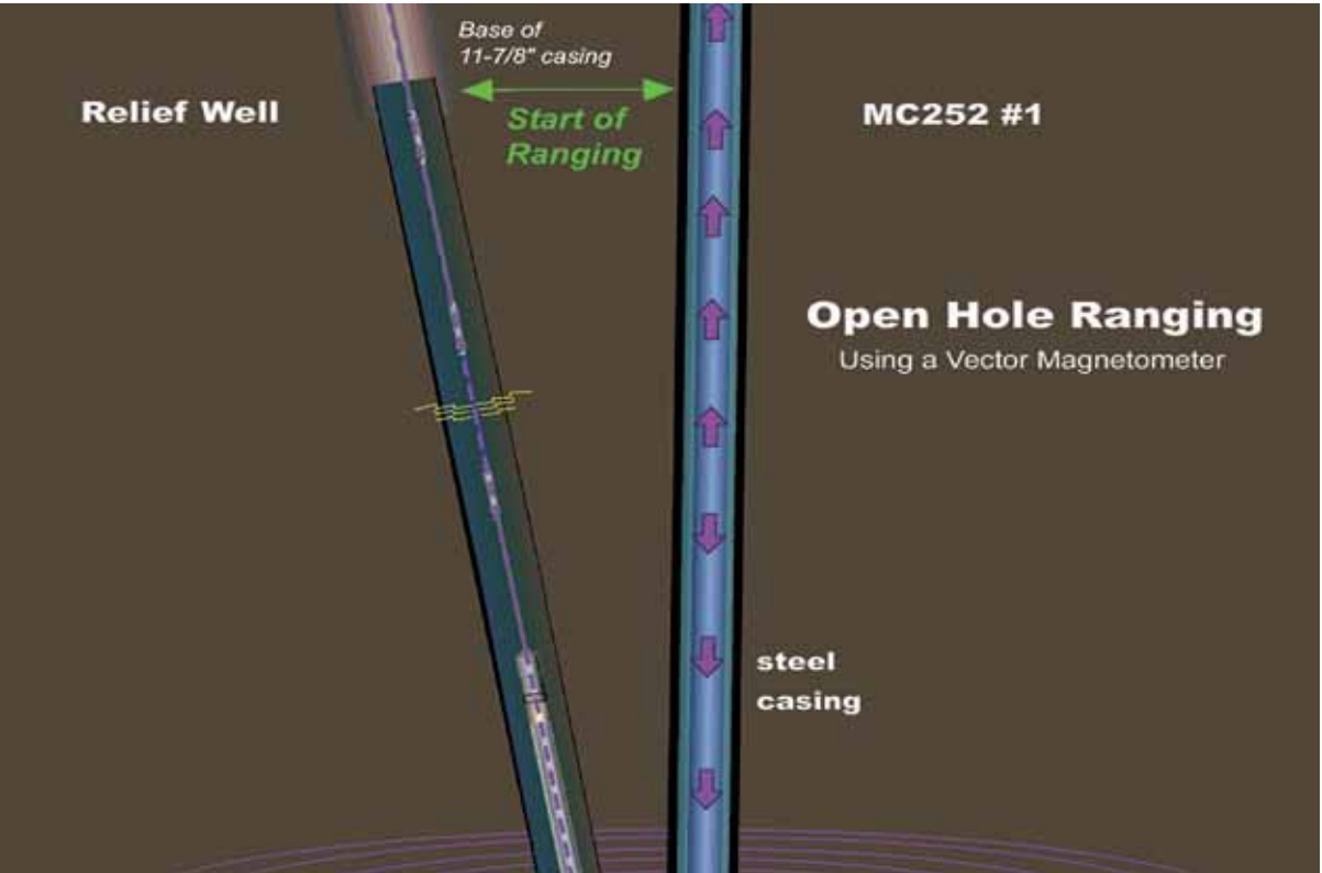
Ranging is the process of locating the existing well casing for intercept. The relief well team initiated the development of two innovative non-wireline technologies that will enable ranging while drilling relief wells.
