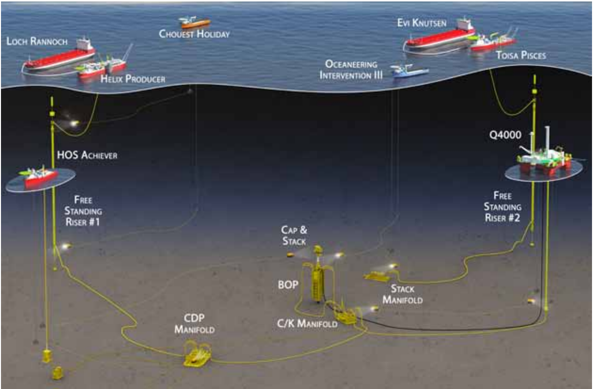
The Containment and Disposal Project team quickly developed a six-month solution for containing hydrocarbon flow with innovations including the first Gulf deployment of free-standing risers and a novel hydrate-inhibition system.
